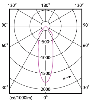
Downlight RS060B G2 LDNR 840 PSR WH-LDD
