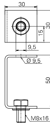
C-bracket
