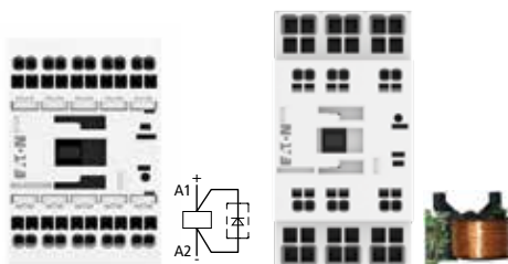
DC / PLC controlled Integrated suppressor circuit
