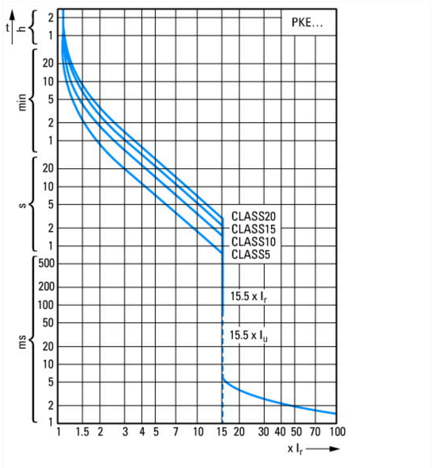
Tripping characteristics
