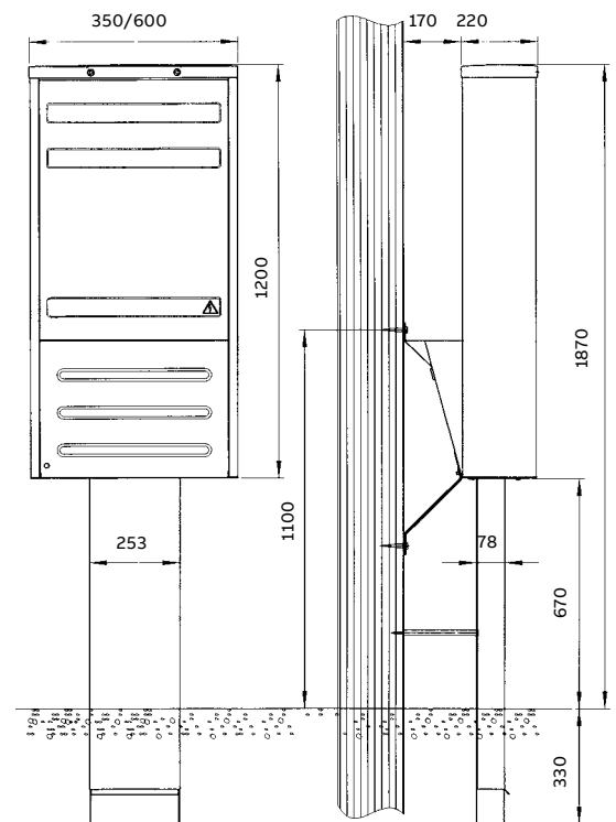
Pole mounted cable distribution cabinets CDCP
