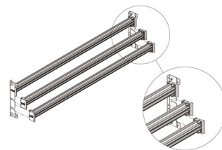
Quick installation, each busbar is lifted into place separately from the front prior to attachment.
