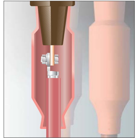
RCAB inline application up to 24 kV
