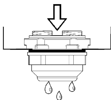
Fitting position
