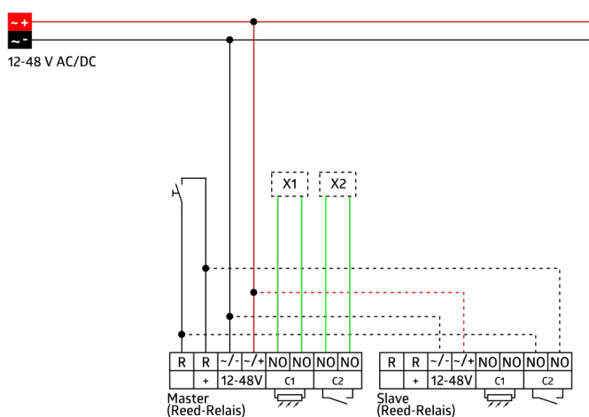
Wiring diagram 92305
