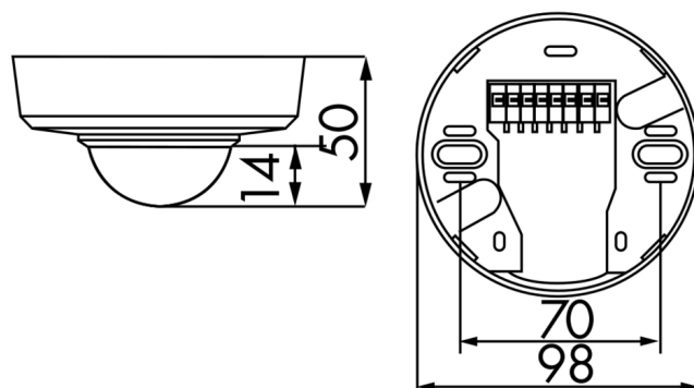
Dimensions 92305
