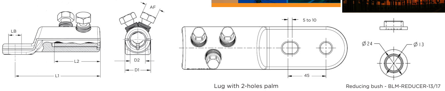
Lug with 2-holes palm
