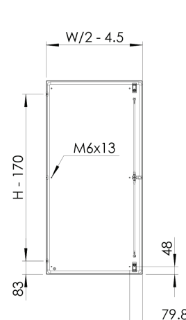
Mounting plate
