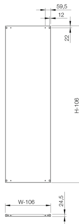
Mounting plate
