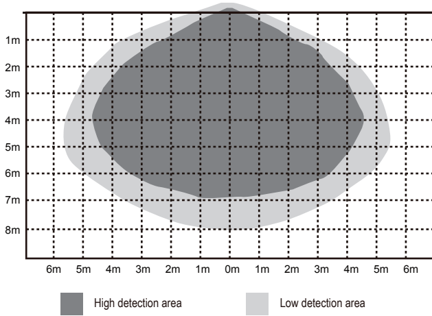
Ceiling mounting height: 3m
