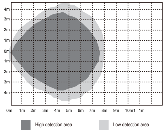
Wall mounting height: 1,5m
