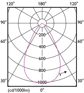
Downlight DN070B 830 24W D200 RD-EU-LDD
