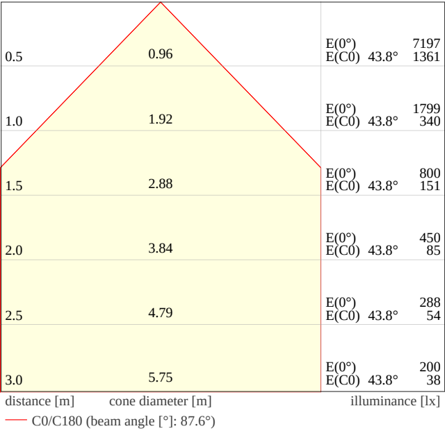
PL CMFT 1200 P 22W 840 U19 3740lm
