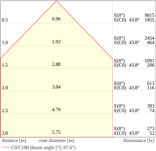
PL CMFT 1200 P 30W ML 840 U19 5100lm
