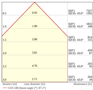
PL CMFT 600 DA P 24W 840 U19 With Inverted Frame
