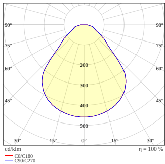
PL CMFT 600 DA P 24W 840 U19 With Circular Cut Out
