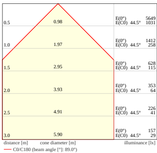
PL CMFT 600 DA P 24W 840 U19 With Circular Cut Out
