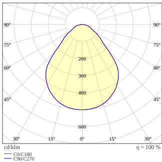
PL CMFT 600 DA P 24W 840 U19 With Inverted Frame
