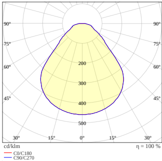
PL CMFT 600 ZB P 33W 830 U19 With Circular Cut Out
