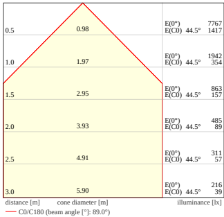
PL CMFT 600 ZB 33W 830 U19 With Circular Cut Out
