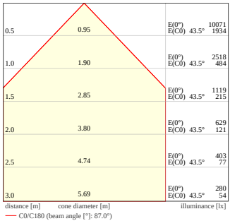
PL CMFT 600 ZB P 33W 830 U19 With Inverted Frame
