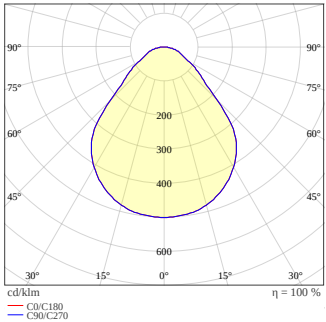
PL CMFT 600 ZB P 33W 830 U19 With Inverted Frame
