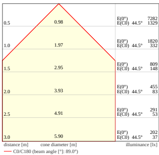
PL CMFT 600 ZB P 33W 940 U19 With Circular Cut Out
