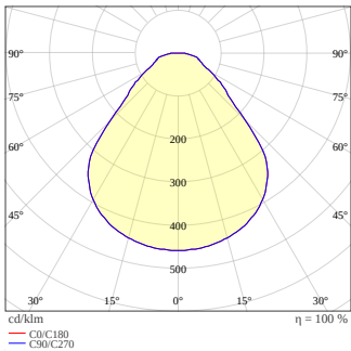
PL CMFT 600 ZB P 33W 940 U19 With Circular Cut Out
