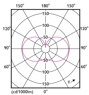
Light Distribution Diagram - CorePro LED HPL/SON M2.6Klm18.3W827E27FR
