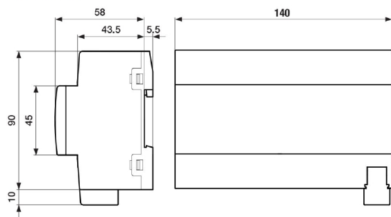
Dimension drawing
