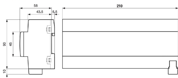
Dimension drawing
