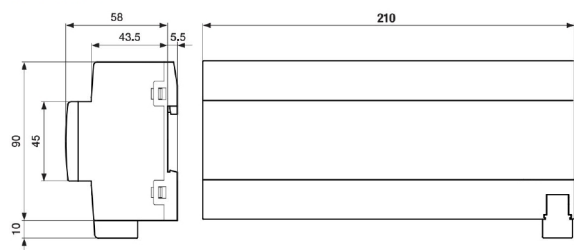
Dimension drawing
